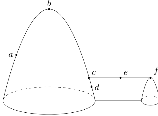
FIGURE 26. The space-time track of the network flow from Figure 25 exhibits several interesting tangent flows, as we discuss below.
