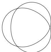
FIGURE 14. One of the Abresch–Langer immersed shrinkers.
