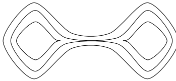
FIGURE 10. Mean convex mean curvature flow (in \mathbb{R}^3 ) as a singular foliation.
