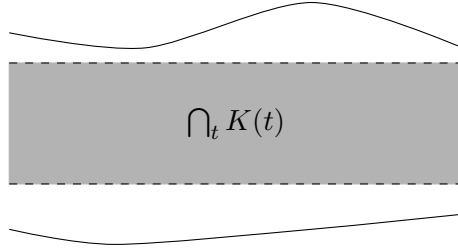
FIGURE 28. The set \cap_t K(t) divides \tilde{\mathcal{M}}(t) into two components
