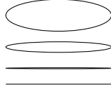
FIGURE 19. Ellipses converging to a line of multiplicity two.
