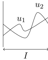
FIGURE 12. Applying the maximum principle to the number of crossings of a graphical flow of curves.
