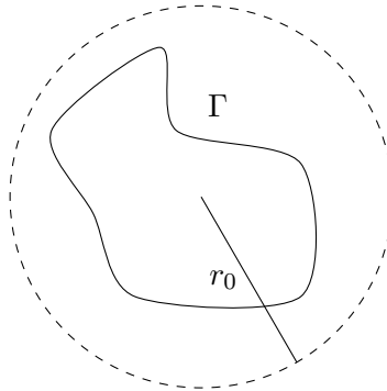
FIGURE 4. The curve \Gamma must disappear before time \frac{r_0^2}{2} , which is when the circle disappears.
