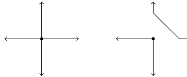
FIGURE 24. Cones with four or more rays cannot be area minimizing, as we could reduce the area of a compact piece, as shown.
