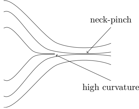
FIGURE 11. Regions of high curvature immediately after the neck-pinch singularity.
