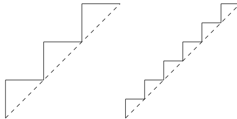
FIGURE 18. Denote M_n the zig-zag curve which is approaching the diagonal.
