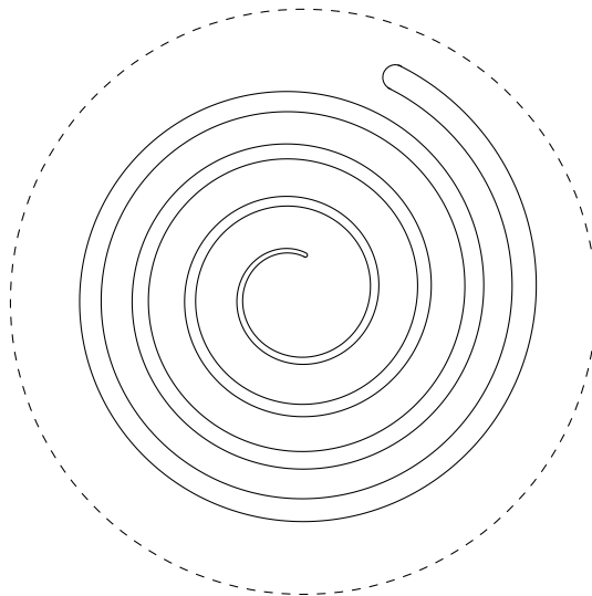
FIGURE 5. Grayson’s theorem implies that this complicated spiraling curve will shrink to a round point. Amazingly, it will do so quite quickly, because it must do so before the dashed circle shrinks away, by the avoidance principle.
