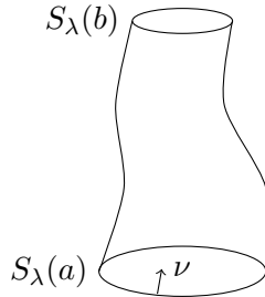
FIGURE 20. The surface M_\lambda(a, b) .
