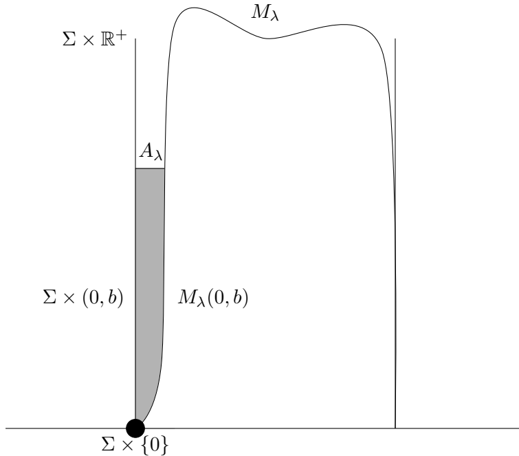
FIGURE 21. Showing that \mu(0) = \mu_{\Sigma \times \mathbb{R}^+} . We will show that the area of the grey region is tending to zero, which implies convergence in the flat norm.
