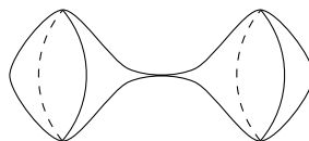
FIGURE 7. At the time of the neck-pinch, most of the surface will remain non-singular, but the diameter of the neck will have shrunk away
