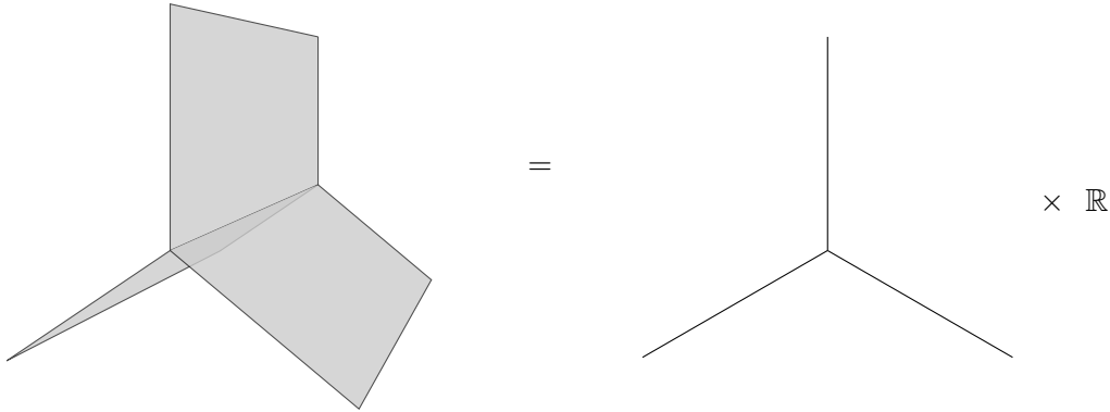
FIGURE 22. The spine (or, equivalently, the set of possible vertex points) of a minimal cone.
