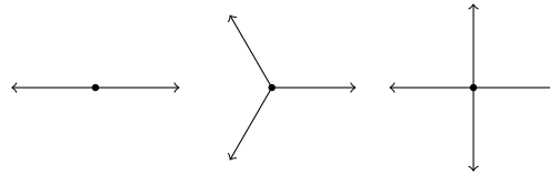
FIGURE 23. Possible 1-dimensional cones. The middle one cannot be a tangent cone to M , as it has boundary point at the origin. The other two are possible cones.
