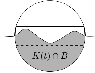
FIGURE 27. The competitor surface in case (1) above is illustrated by a bold line.
