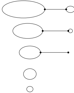
FIGURE 25. An example of a Brakke flow of curves (known as the network flow ).
