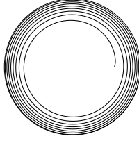
FIGURE 13. It is possible to construct a function f : \mathbb{R}^2 \rightarrow \mathbb{R} so that the gradient flow of f spirals into an entire circle (and in particular does not have a unique limit as t \rightarrow \infty ).
