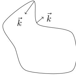
FIGURE 1. An embedded curve \Gamma \subset \mathbb{R}^2 and its curvature vector \vec{k} .
