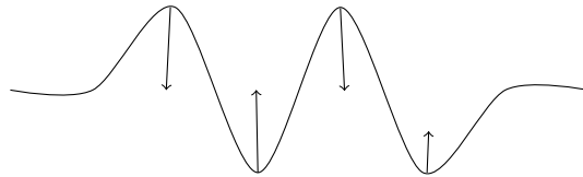
FIGURE 2. This illustrates the short time smoothing property of curve shortening flow. The curvature vector points in a direction which serves to smooth the curve out.
