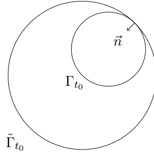
FIGURE 3. If \tilde{\Gamma} encloses \Gamma and the curves are originally disjoint, then if \tilde{\Gamma}_t were to touch \tilde{\Gamma}_t for some t > 0 , then if t_0 is the time of first contact, the point of contact will look like this diagram. In particular \vec{k}_{\tilde{\Gamma}_{t_0}} \cdot \vec{n} \leq \vec{k}_{\Gamma_{t_0}} \cdot \vec{n} at this point of contact. If the inequality was strict, this would immediately yield a contradiction, as it would imply that they must have crossed for t = t_0 - \epsilon , contradicting the choice of t_0 . In general, we must reason using the maximum principle to rule this situation out.
