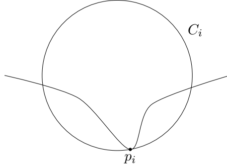
FIGURE 15. The circle C_i must intersect \Gamma_i(t) in at least 3 points.
