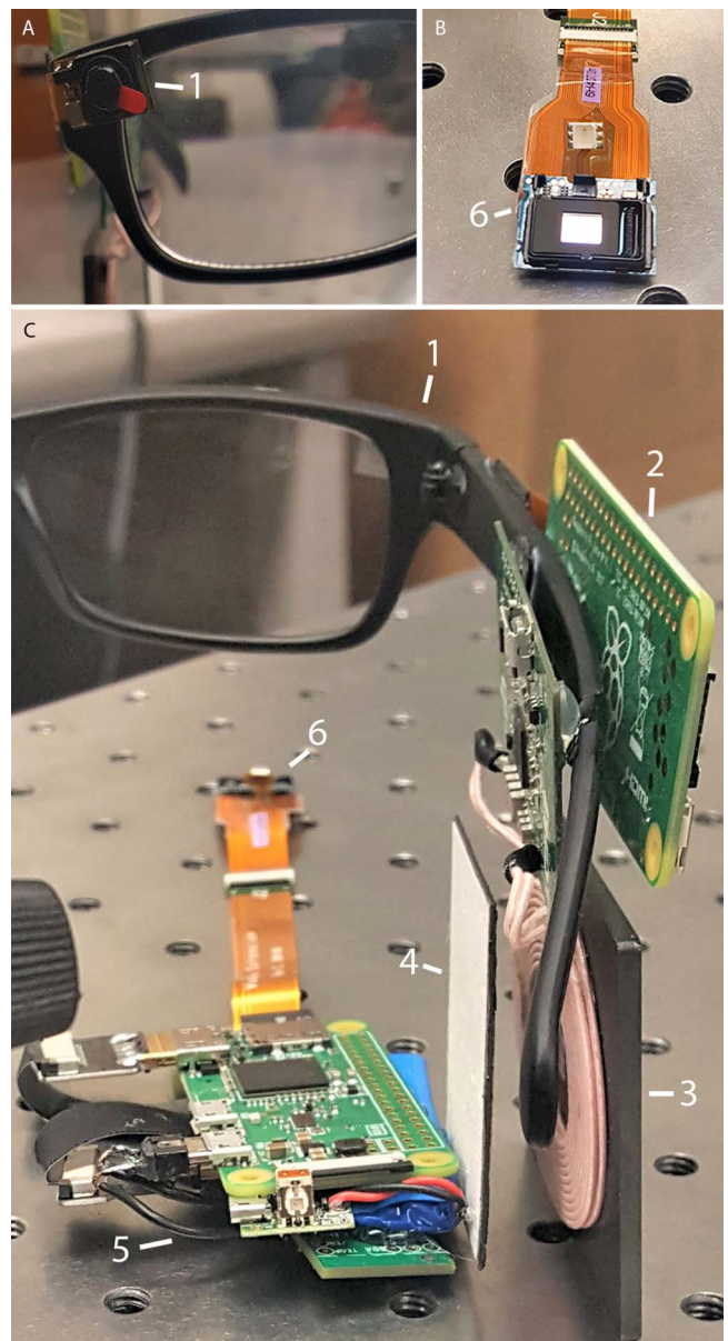
FIGURE 4. Prototype of the intraocular display electronics. A, External camera (1). B, Microdisplay (6). C, A camera (1) captures video, which is encoded by a processor (2), which sends the data and power through a transmission coil (3) to a receiver coil (4). The signal is then decoded by another processor (5), and the recovered video is displayed by the microdisplay (6).
