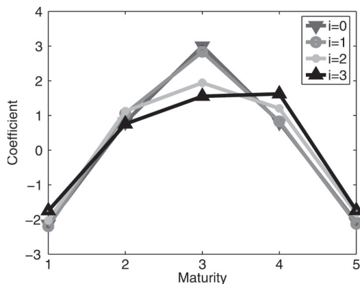
FIGURE 3. COEFFICIENTS IN REGRESSIONS OF AVERAGE (ACROSS MATURITY) EXCESS RETURNS ON LAGGED FORWARD RATES, \bar{r}_{t+1} = \boldsymbol{\gamma}^\top \mathbf{f}_{t-i/12} + \varepsilon_{t+1}
