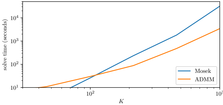
Fig. 5 The solve time as a function of graph size.
