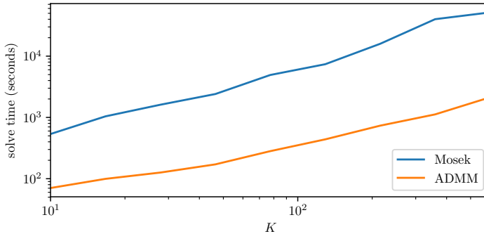
Fig. 6 The solve time as a function of number of scenarios.
