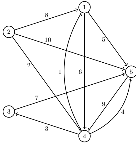
Fig. 1 The graph of the illustrative example.
