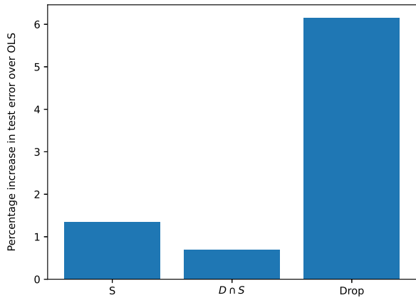
Fig. 2 Excess test error in the Airbnb price prediction experiment
