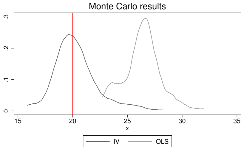
Figure shows the distribution of the estimated parameter under each method. IV estimate (mean/sd) = 20.3 ( 2.1). OLS estimate (mean/sd) = 26.3 ( 1.7). Number of iterations = 100. The red line shows the true value of theta.
