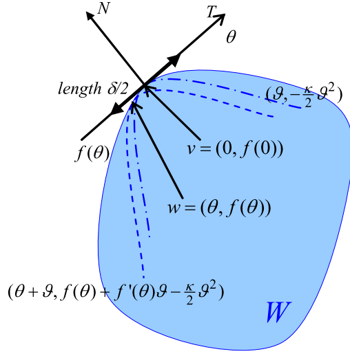
FIGURE O4.—Set W and the points (\theta + \vartheta, f(\theta) + f'(\theta)\vartheta - \frac{\kappa}{2}\vartheta^2) .
