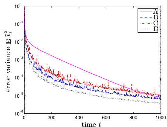
Figure 3: Estimation error variance at 4 nodes, each being a representative from the four regions A, B, C and D (big black dots in Figure 2).
