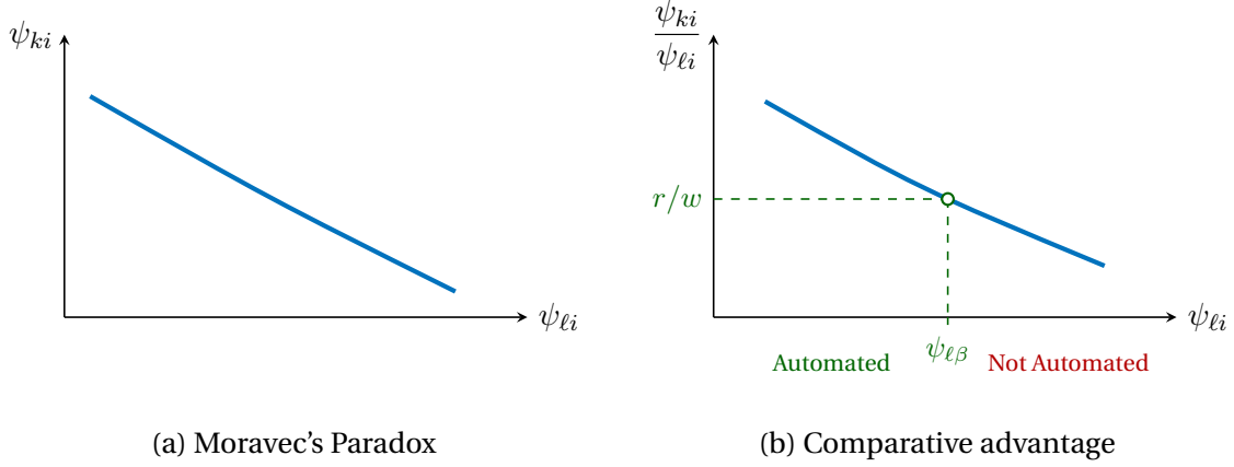
Figure 3: Moravec's Paradox
