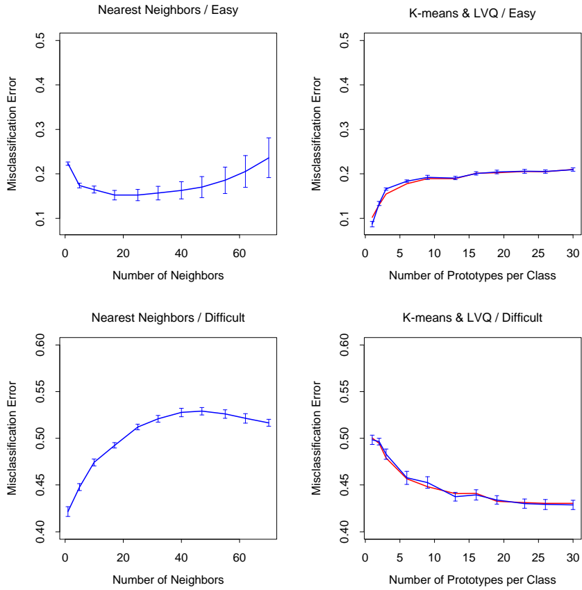
FIGURE 13.5. Mean \pm one standard error of misclassification error for nearest-neighbor, K -means (blue) and LVQ (red) over ten realizations for two simulated problems: “easy” and “difficult,” described in the text.
