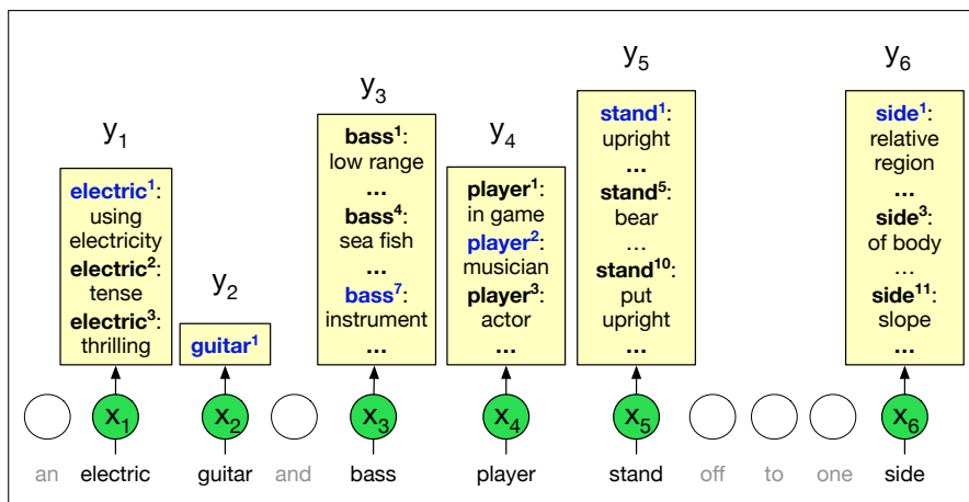
Figure 10.7 The all-words WSD task, mapping from input words ( x ) to WordNet senses ( y ). Figure inspired by Chaplot and Salakhutdinov (2018) .
