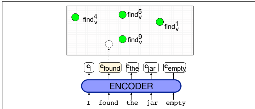
Figure 10.8 The nearest-neighbor algorithm for WSD. In green are the contextual embeddings precomputed for each sense of each word; here we just show a few of the senses for find . A contextual embedding is computed for the target word found , and then the nearest neighbor sense (in this case find v 9 ) is chosen. Figure inspired by Loureiro and Jorge (2019).
