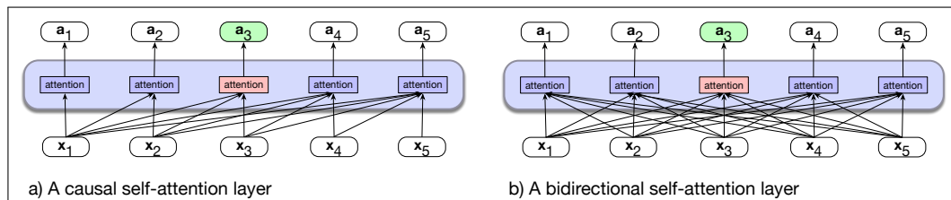
Figure 10.1 (a) The causal transformer from Chapter 8, highlighting the attention computation at token 3. The attention value at each token is computed using only information seen earlier in the context. (b) Information flow in a bidirectional attention model. In processing each token, the model attends to all inputs, both before and after the current one. So attention for token 3 can draw on information from following tokens.
