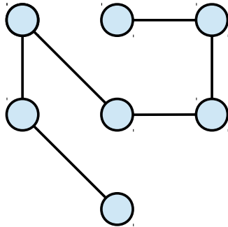
7 Nodes, 6 Edges
