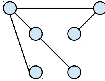
6 Nodes, 5 Edges
