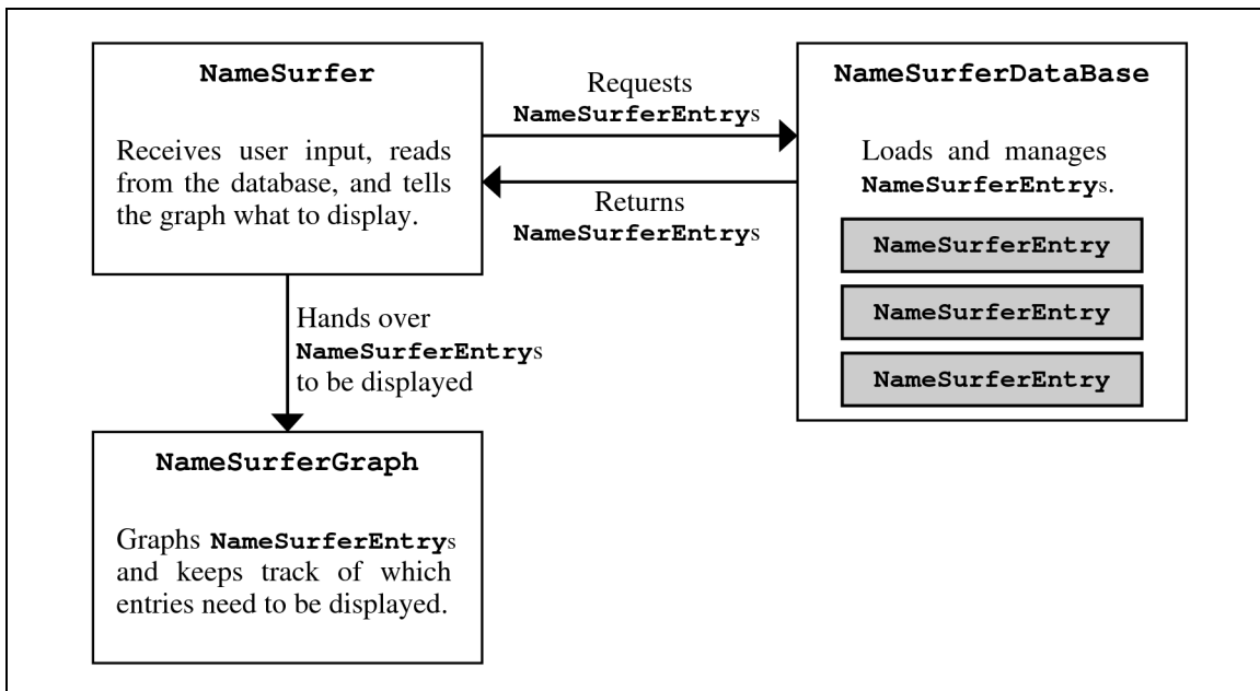
Figure 2. Module structure for the NameSurfer application
