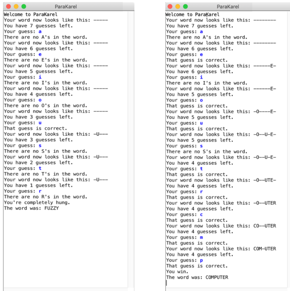
Figure 1. Two sample runs of the ParaKarel program (console only)
