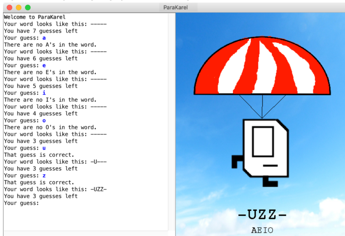
Figure 4. Midway through a graphical ParaKarel game
