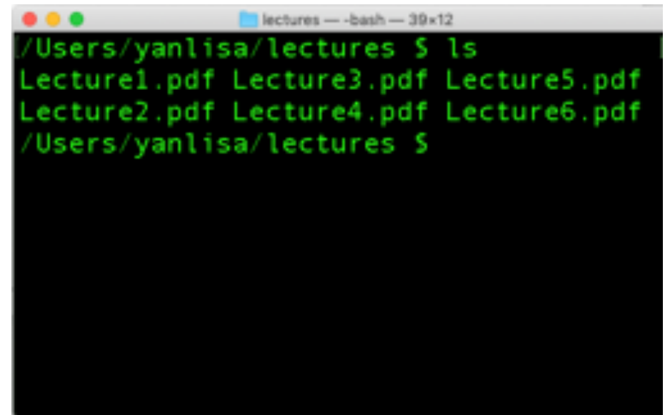
Text-based interface
