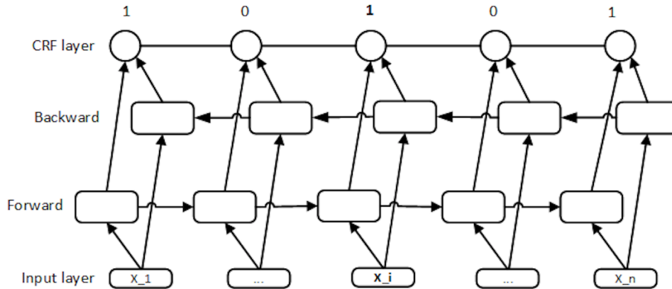
Figure 1: Thai Segmentation Model using BiLSTM-CRF architecture or BiGRU-CRF architecture. [6].
