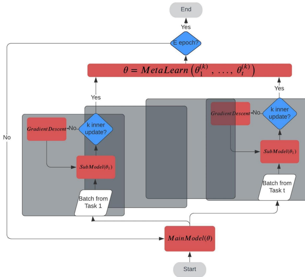
Figure 3: MAML architecture
