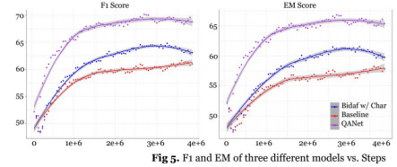
Fig 5. F1 and EM of three different models vs. Steps
