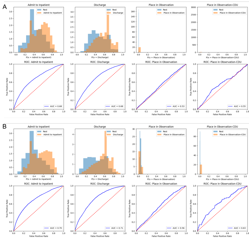
Figure 8: Histograms and ROC curves of each disposition class. Classification results after fine-tuning pretrained model (A) ClinicalBERT in method 1, trained only on text reports (B) ClinicalBERT in method 3, trained on text reports and result of the zero-shot labeler.
