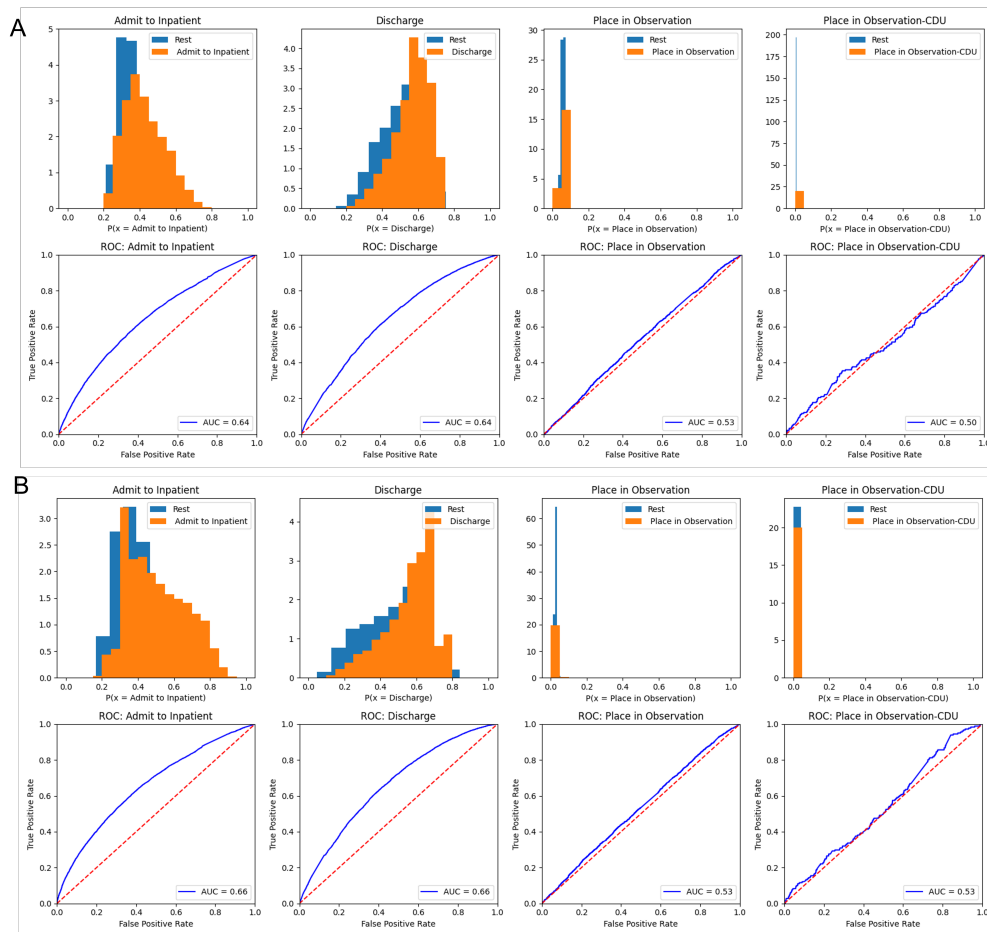
Figure 6: Histograms and ROC curves of each disposition class. Classification results after fine-tuning pretrained model (A) BERT in method 1, trained only on text reports (B) BERT in method 3, trained on text reports and result of the zero-shot labeler.
