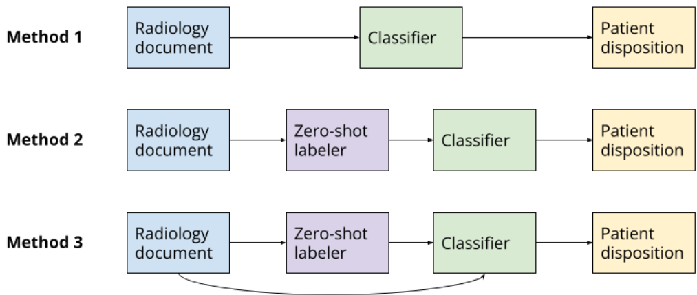
Figure 1: Experiments conducted in the project.
