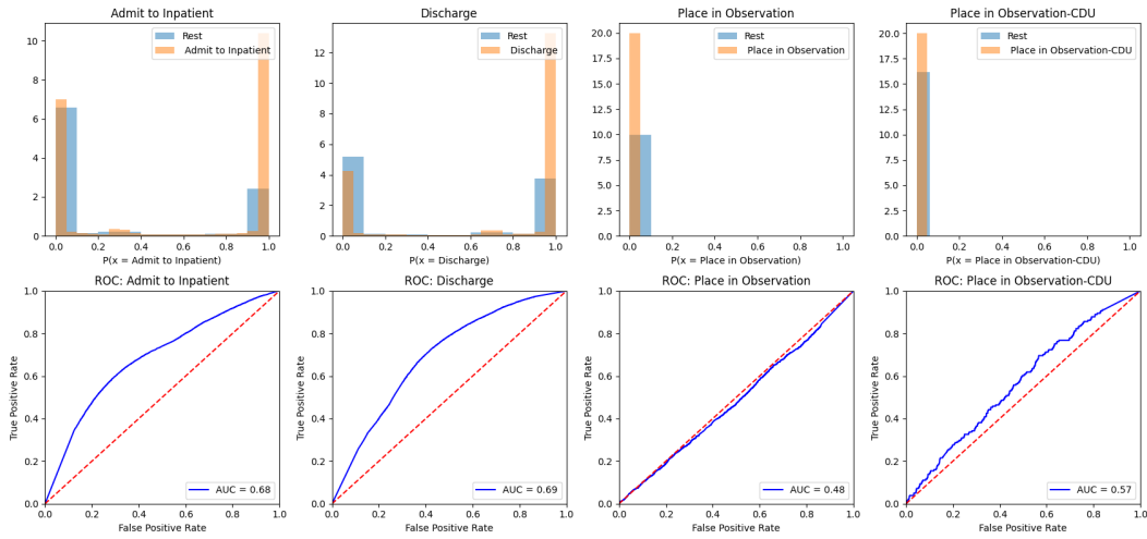
Figure 5: Histograms and ROC curves of each disposition class. Classification results from multilayer perceptron model trained on the 39 extracted labels. Like in other experiments, the model has useful ROC for the first two common classes, while basically ignoring the rare "Place in Observation" classes
