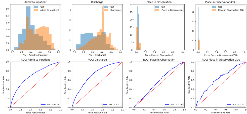
Figure 4: Histograms and ROC curves of each disposition class. Classification results after fine-tuning pretrained model ClinicalBERT.
