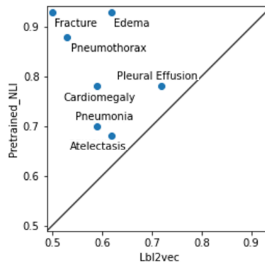
Figure 2: Comparing AUC from Table 2
