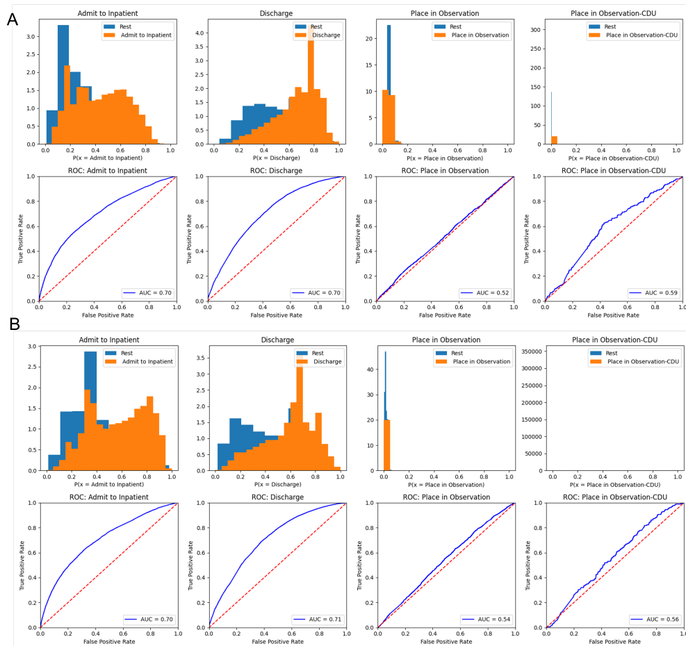
Figure 7: Histograms and ROC curves of each disposition class. Classification results after fine-tuning pretrained model (A) BIO BERT in method 1, trained only on text reports (B) BIO BERT in method 3, trained on text reports and result of the zero-shot labeler.
