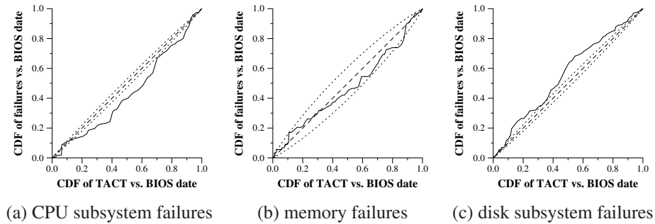
Figure 13. P-P plots of failure count versus TACT, relative to BIOS date
