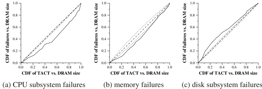
Figure 12. P-P plots of failure count versus TACT, relative to DRAM size
