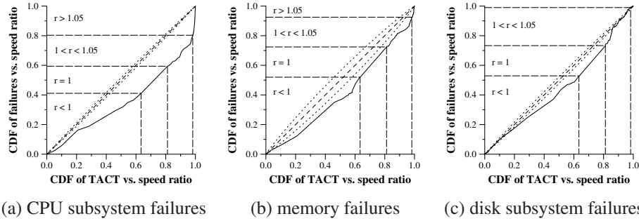
Figure 11. P-P plots of failure count versus TACT, relative to the ratio of CPU speed to rated speed
