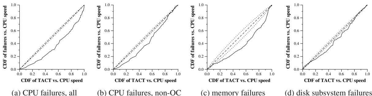
Figure 9. P-P plots of failure count versus total aggregate CPU seconds (TACT), relative to CPU speed. The dashed line y = x shows where a perfectly independent plot would lie. The dotted lines outline a 99% confidence envelope for independence. Whereas (a), (c), and (d) show all machines for which CPU speed could be determined, (b) shows only machines whose CPU speeds are no more than 0.5% over rated speed.
