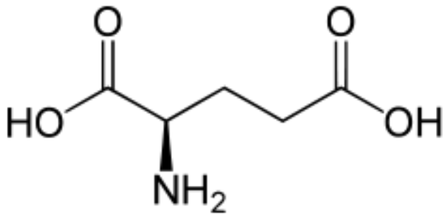
Glutamic acid
