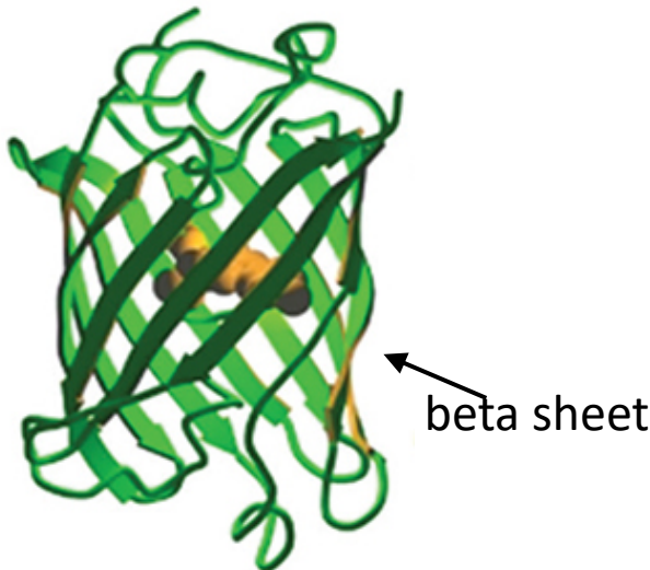
Green Fluorescent Protein
