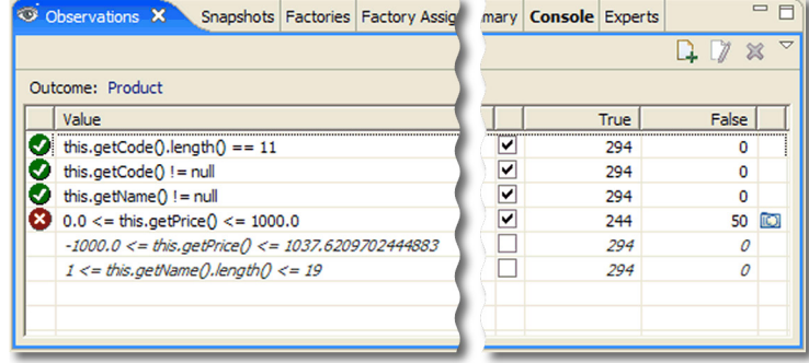
(b) Observations View
