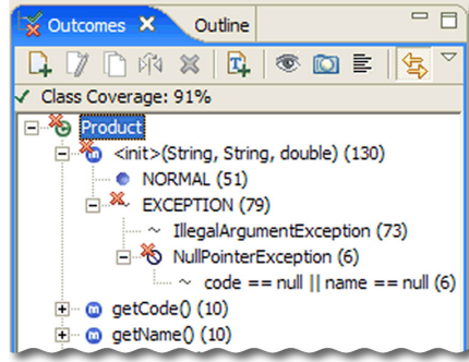
(a) Outcomes View
