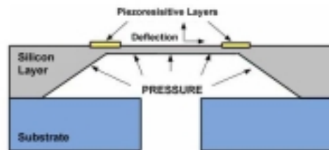
Figure 6. Schematic illustration of a piezoresistive pressure sensor.
