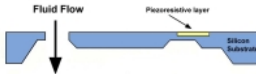
Figure 36. Micromachined mechanical (drag-force) flow sensor [39].
