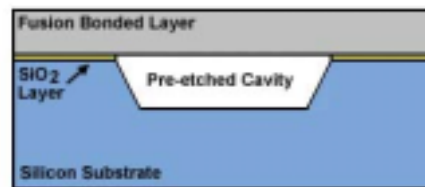
Figure 23. Formation of sealed cavity using fusion bonding
