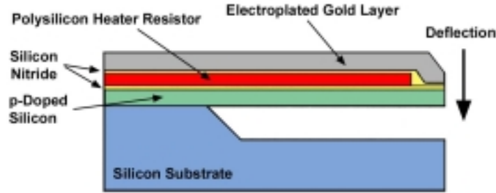
Figure 33. Example of a MEMS thermal bimorph actuator [34].
