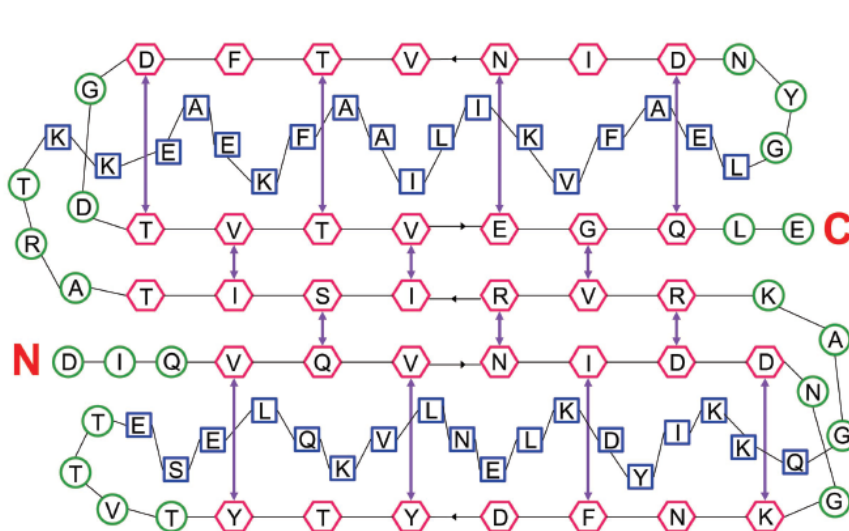
Fig. 1. A two-dimensional schematic of the target fold (hexagon, strand; square, helix; circle, other). Hydrogen bond partners are shown as purple arrows. The amino acids shown are those in the final designed (Top7) sequence.
