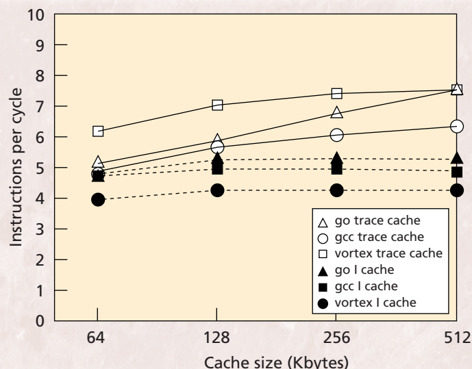
Figure 2. Performances of various fetch mechanisms as the size of the cache structure increases. At 512 Kbytes, the trace cache continues to gain performance.
