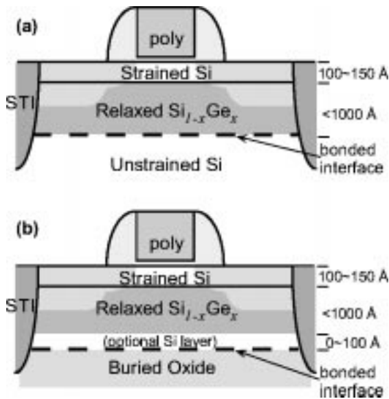
Fig. 13. Structures of (a) bulk and (b) SOI strained-Si MOSFET's with a thin relaxed \text{Si}_{1-x}\text{Ge}_x layer.
