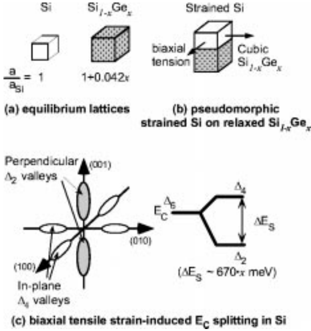
Fig. 1. Schematic illustrations of (a) equilibrium lattices, (b) pseudomorphic strained Si on relaxed Si 1-x Ge x , and (c) strain-induced conduction band splitting in Si.
