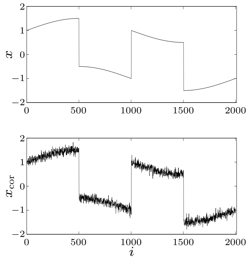
original signal x and noisy signal x_{\text{cor}}
