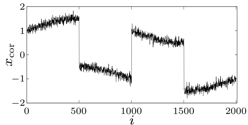
original signal x and noisy signal x_{\text{cor}}
