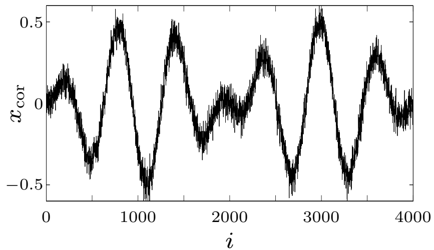
original signal x and noisy signal x_{\text{cor}}
