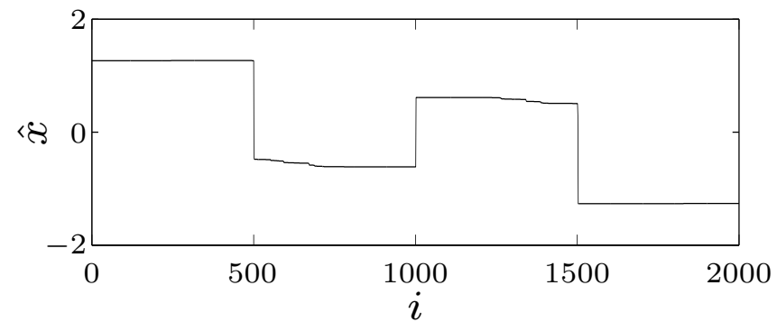
three solutions on trade-off curve \|\hat{x} - x_{\text{cor}}\|_2 versus \phi_{\text{tv}}(\hat{x})
