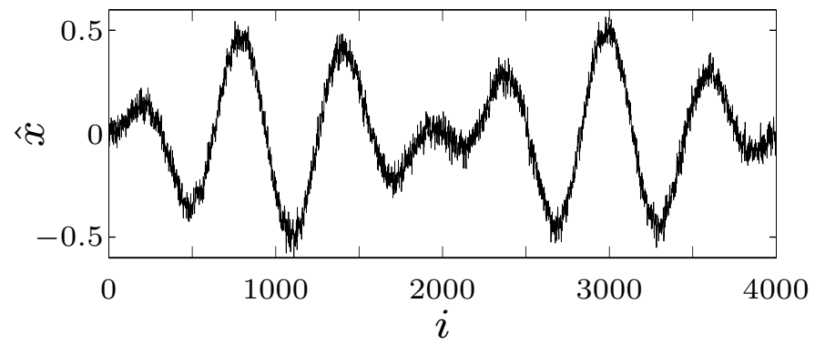
three solutions on trade-off curve \|\hat{x} - x_{\text{cor}}\|_2 versus \phi_{\text{quad}}(\hat{x})
