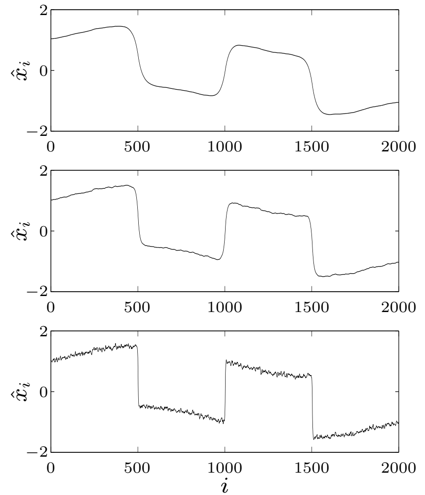
three solutions on trade-off curve \|\hat{x} - x_{\text{cor}}\|_2 versus \phi_{\text{quad}}(\hat{x})
