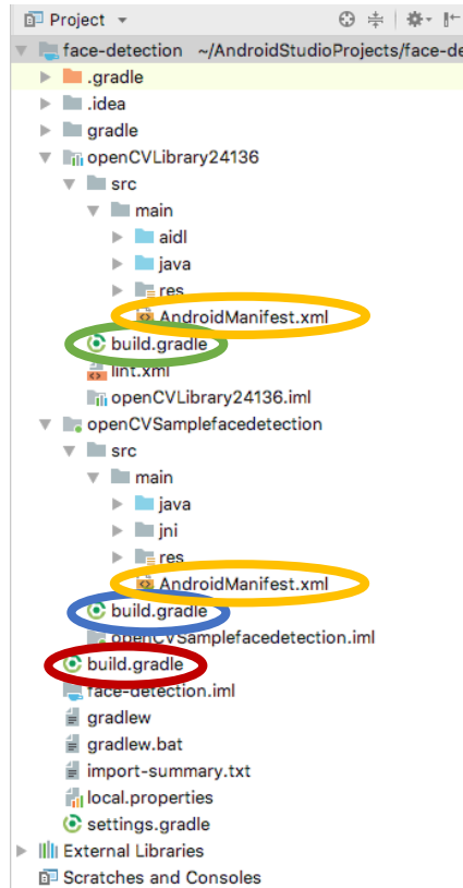
Figure 2. Screenshot of the “Project” panel in Android Studio.
