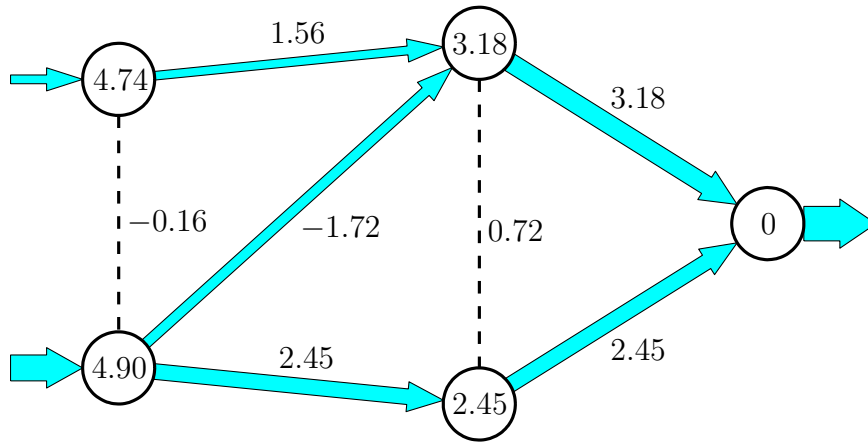
Figure 10: Optimal network flows plotted as pipes with arrows, and the widths of the pipes are proportional to the flows x_j . The numbers at each node i are the optimal dual variables \nu_i , and the numbers at each link j are \Delta\nu_j , i.e. , the differences between the dual variables at their two incident nodes (along the reference direction given in figure 9). Link 1 and 5 have zero flow because their corresponding \Delta\nu_j are smaller than the threshold 1, see figure 8.
