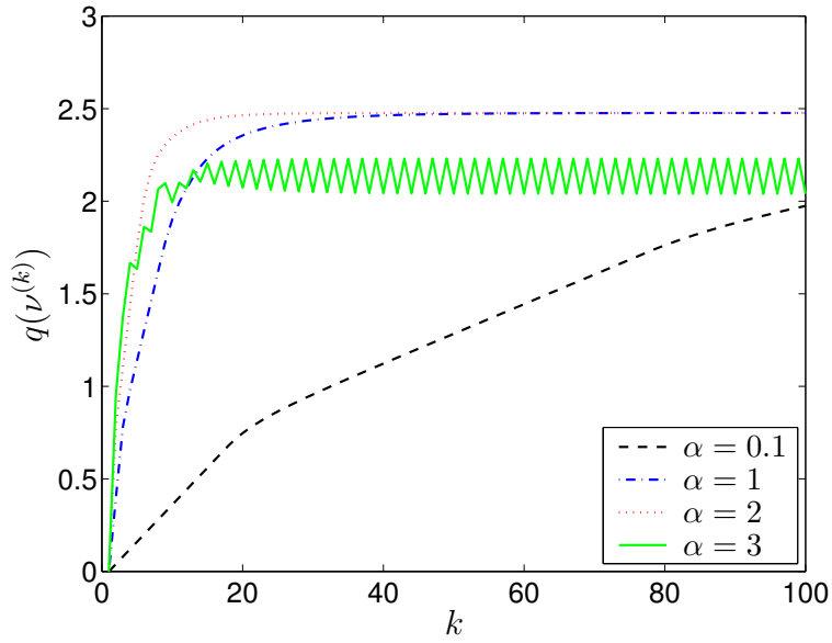
Figure 11: Dual function value versus iteration number k , for the subgradient method with the constant stepsize rule. For \alpha = 1 and 2, the dual function comes very close to the optimal value 2.48 after about 40 iterations.
