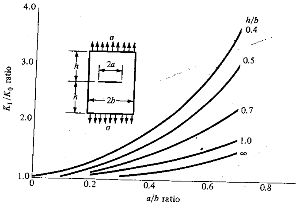
FIGURE 5-19 ...ing a central crack longitudinal tension.
