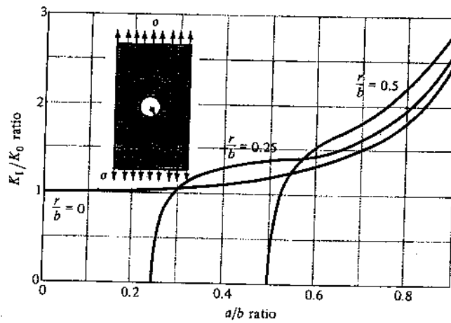
FIGURE 5-24 Plate in tension containing a circular hole with two cracks.
