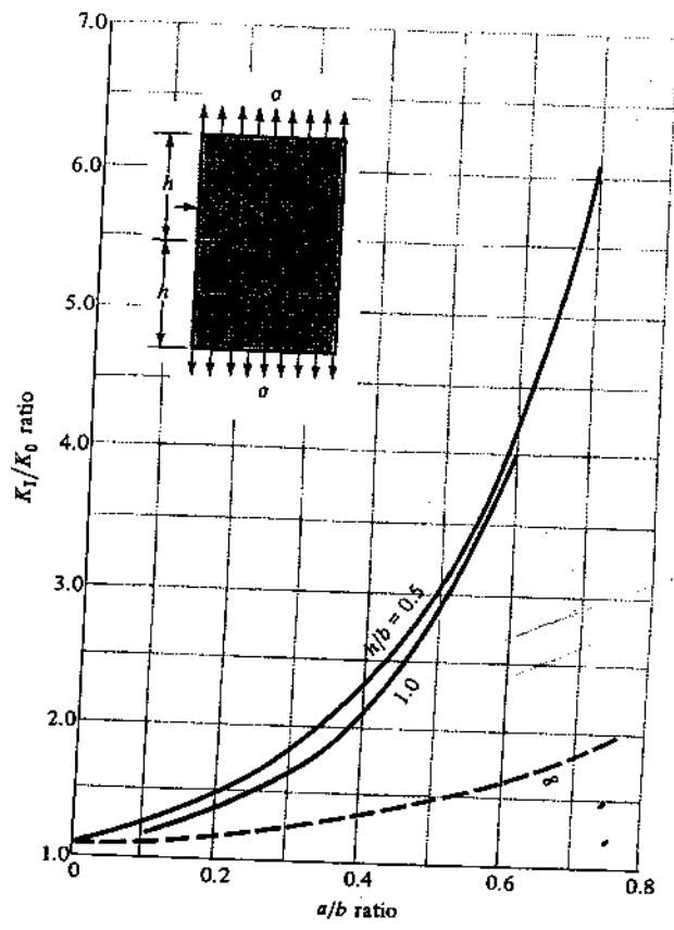
FIGURE 5-22 Plate loaded in longitudinal tension with a crack at the edge; for the solid curve there are no constraints to bending; the dashed curve was obtained with bending constraints added.
