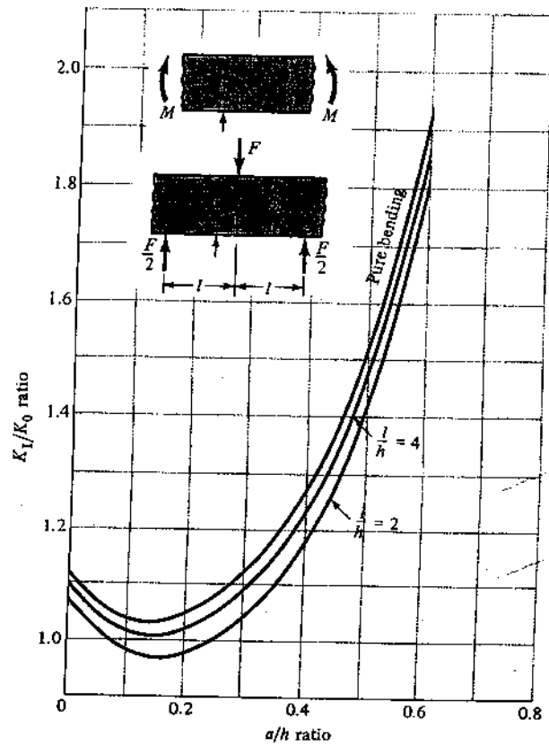
FIGURE 5-23 Beams of rectangular cross section having an edge crack.
