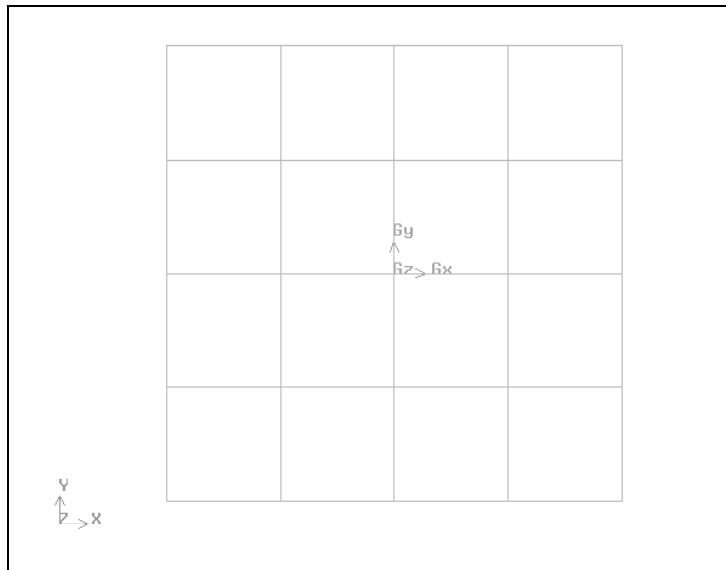
Figure 2-2: 4x4 grid to be used for creating vertices
