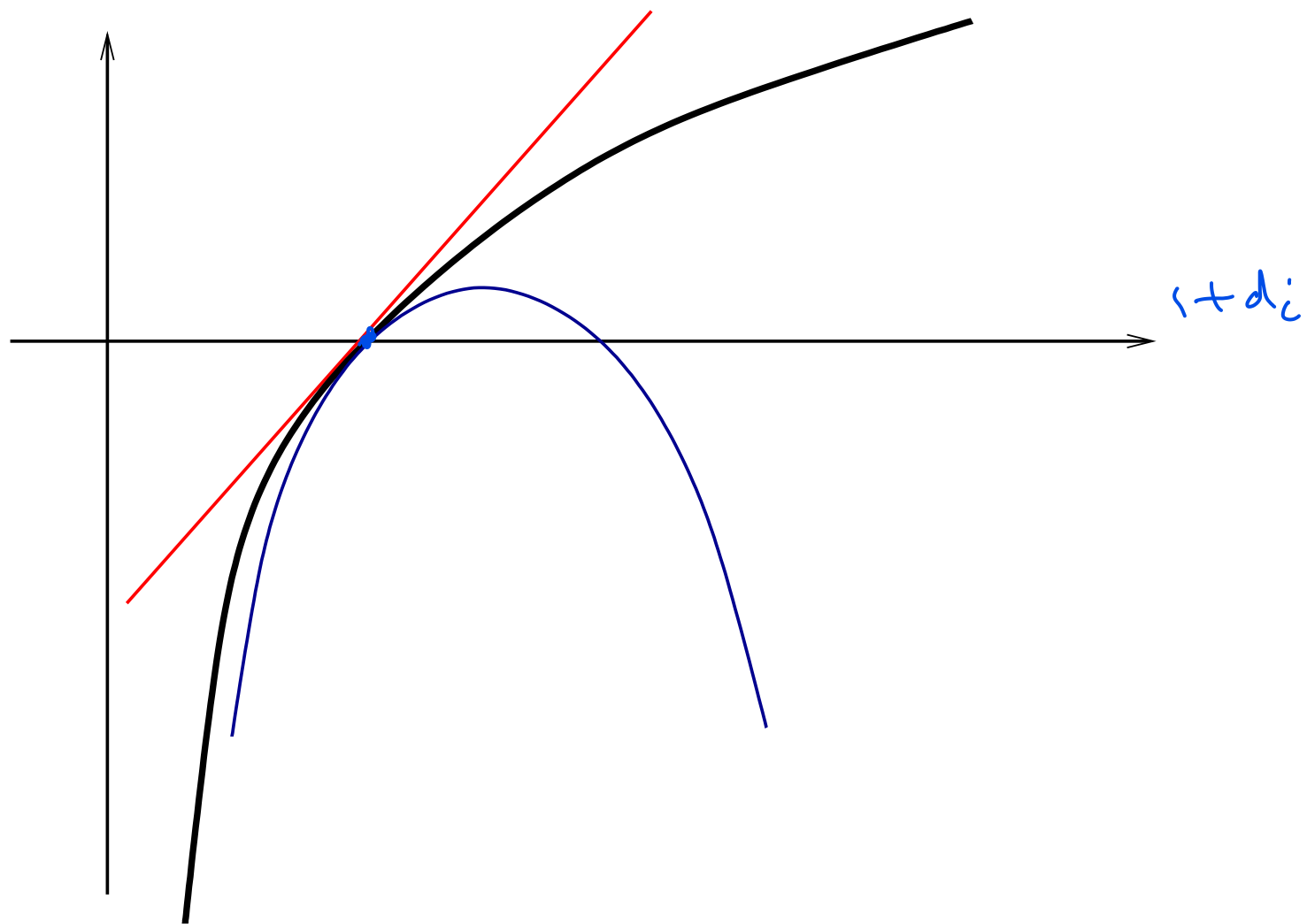
Figure 1: Logarithmic approximation by linear and quadratic functions
