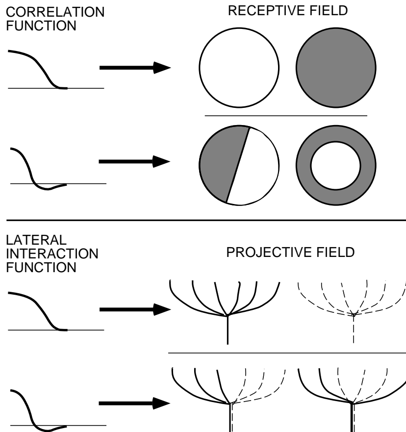
FIGURE 1.4. Schematic of the outcome of semi-linear correlation-based development.
