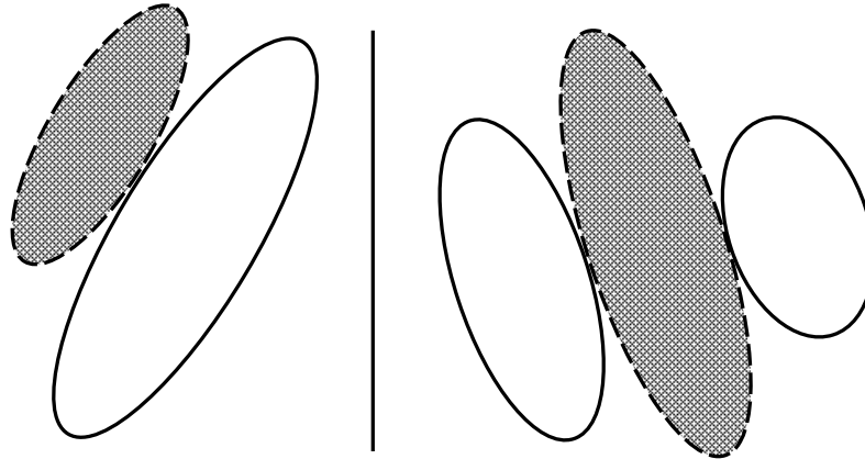
FIGURE 1.3. Two examples of simple cell receptive fields (RFs). Regions of the visual field from which a simple cell receives ON-center (white) or OFF-center (dark) input are shown. Note: Ocular dominance columns (Fig. 1.2) represent an alternation, across cortex, in the type of input (left- or right-eye) received by different cortical cells; while a simple cell RF (this figure) represents an alternation across visual space in the type of input (ON- or OFF-center) received by a single cortical cell.
