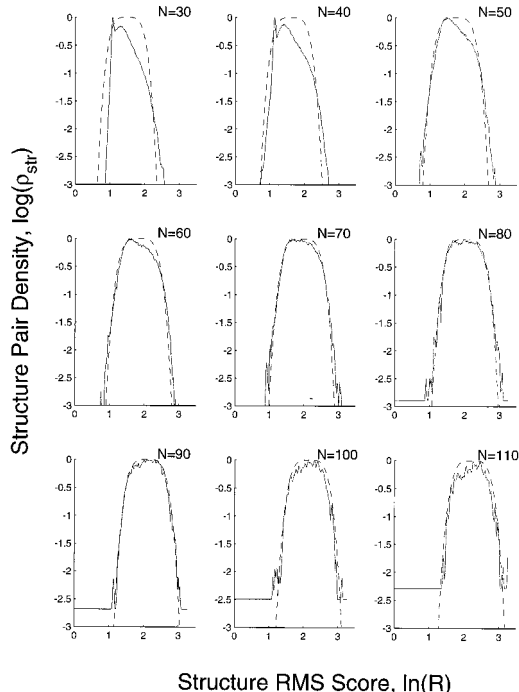
FIG. 5. The fit to the structure pair density by using the rms score. The observed, \log(\rho_{\text{str}}^0) , and calculated, \log(\rho_{\text{str}}^c) , structure pair density distributions are plotted against the rms score \ln(R) for different numbers of aligned residues, N . The observed structure pair density, which is derived from pairs in different classes, is clearly not an extreme-value distribution because it is symmetrical about the maximum value and falls off faster than a linear function with increasing Z . In fact, it is best fit by \exp(-Z^4) . The calculated distribution obtained with a five-parameter fit (dashed line) is a good fit when the number of aligned residues exceeds 50.
