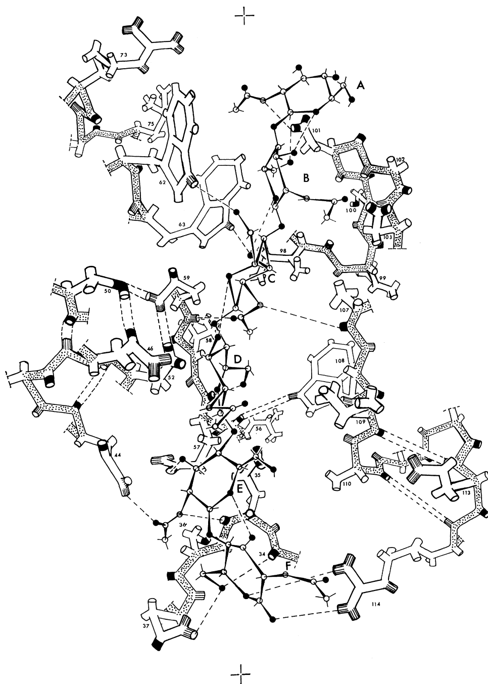
FIG. 7.—Atomic arrangement in the lysozyme molecule in the neighborhood of the cleft with a hexa- N -acetylchitohexaose shown bound to the enzyme. The main polypeptide chain is shown speckled and NH and O atoms are indicated by line and full shading, respectively. Sugar residues A , B , and C are as observed in the binding of tri- N acetylchitotriose (and \beta - N -acetylglucosamine for residue C ). Residues D , E , and F occupy positions inferred from model building. It is suggested that the linkage hydrolyzed by the action of the enzyme is between residues D and E .
