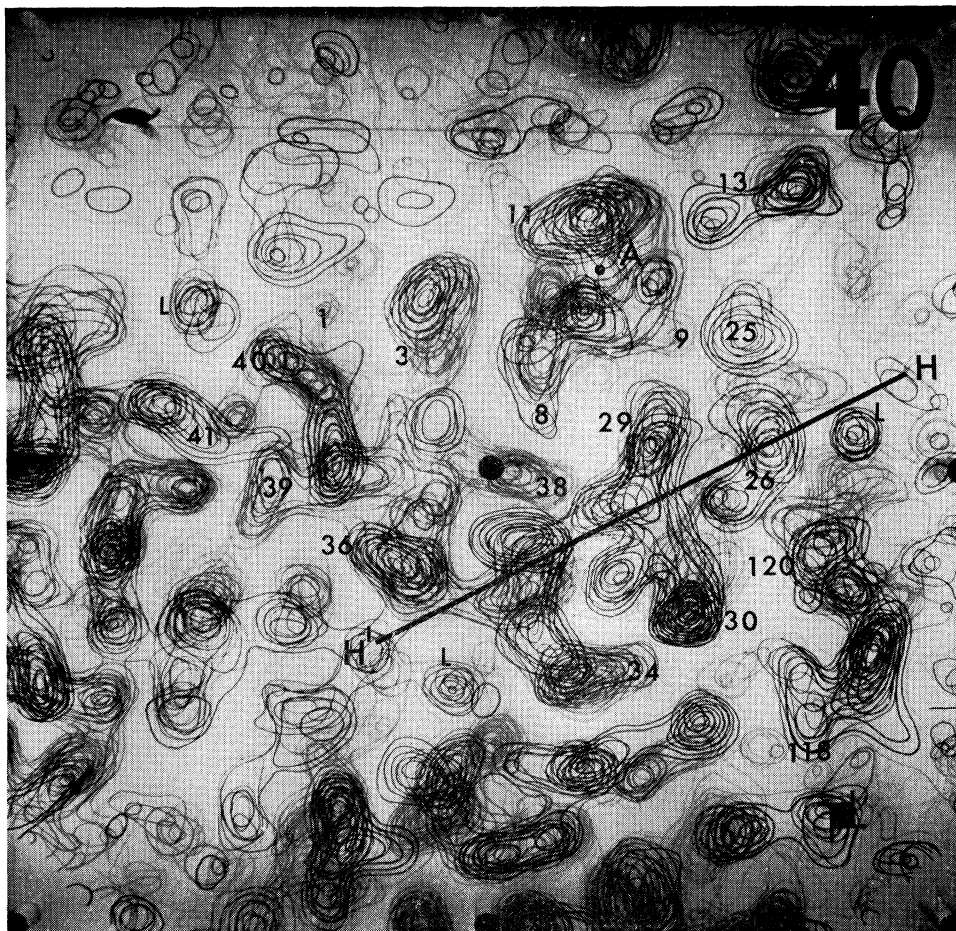
Fig. 2.—The sections Z = 40-49/60 of the 2\text{-\AA} electron density map. Contours at intervals of 0.25\text{ e\AA}^{-3} . HH' shows the course of a length of helix lying in the plane of the sections. A indicates a length of helix more nearly normal to the sections. The densities corresponding to a number of amino acid side chains are numbered in accordance with Fig. 1 and three probable \text{Cl}^- ions are labeled L .
