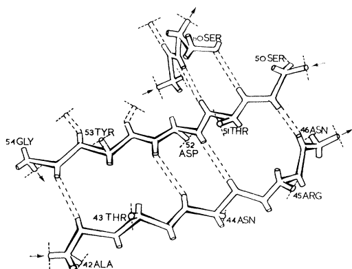
FIG. 3.—The region of antiparallel pleated sheet.
