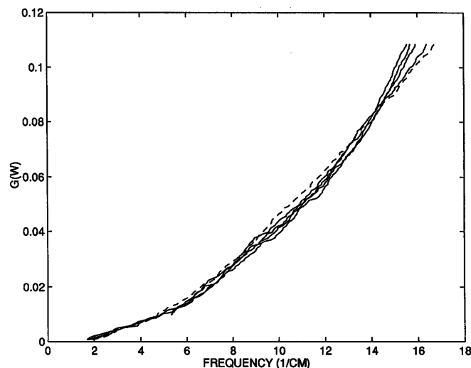
FIG. 1. The fraction of the total number of modes up to frequency \omega ( \text{cm}^{-1} ) for the slowest 150 modes of the G-actin:ADP: \text{Ca}^{++} system. The dashed line pertains to data obtained using the L79 potential, while the four solid curves are obtained using R_c values of 1.1, 1.5, 2.0, and 2.5 Å. The R_c = 1.1 Å curve is nearest the dashed line at higher frequencies, with the fit progressively worsening for the higher cutoff values.
