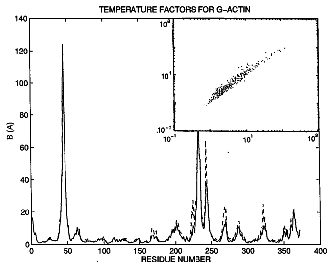
FIG. 3. Comparison of theoretical temperature factors, B , obtained with the L79 potential (dashed curve) and the potential of Eq. (1), for the G-actin:ADP: \text{Ca}^{++} system. The contributions of the 30 slowest modes are included. The inset shows the scatter plot of the two data sets: the standard potential along the ordinate, and the current simplified potential along the abscissa.
