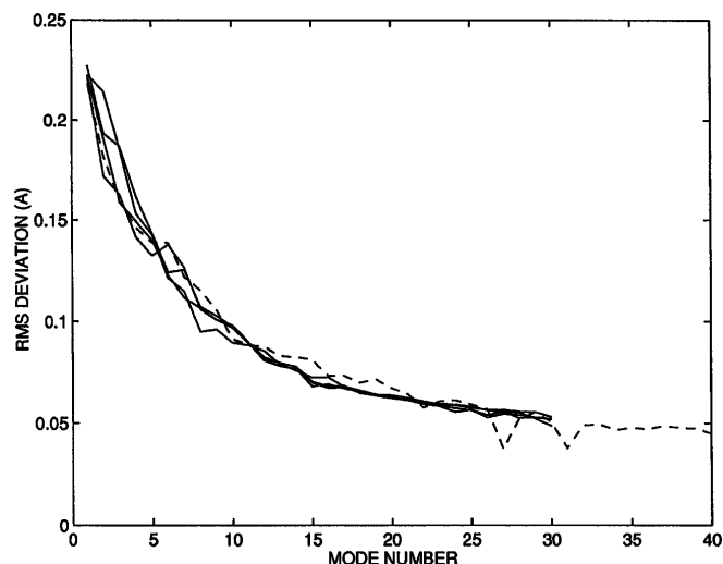
FIG. 2. The rms deviation of all mainchain C_\alpha atoms per mode, for the slowest 30 modes. The dashed line refers to data obtained using the L79 potential, and the four solid curves are obtained with the same cutoff values, R_c , as in Fig. 1. The rms fluctuations due to the first four modes contribute over 50% to the total rms deviations of all C_\alpha due to all modes [8]. There is no obvious improvement in choosing one particular cutoff parameter according to these data.
