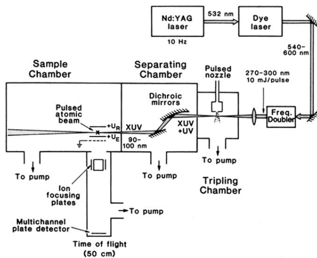
FIG. 1. Experimental setup.
