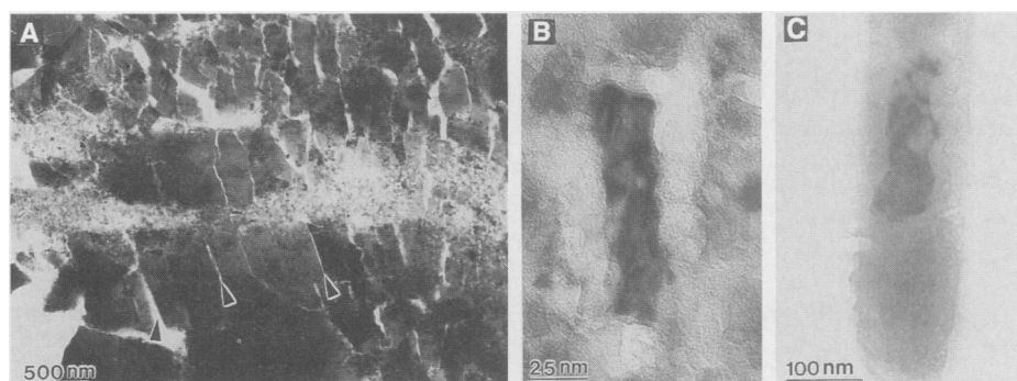
Fig. 5. TEM images of a thin section showing the morphology of the Fe-sulfide phases present in ALH84001 and a terrestrial soil sample. Iron sulfide phase (greigite?— \text{Fe}_3\text{S}_4 ) is located in a magnetite-poor region separate and distinct from the magnetite-rich rims (Fig. 3A, arrow II). (A) TEM of a thin section showing a cross section of a single carbonate crystal (large black regions; the apparent cleavage features are due to knife damage by ultramicrotomy). A vein of fine-grained carbonate (light gray) is observed within the large carbonate crystal. Possibly greigite and secondary magnetite (fine, dark crystals) have been precipitated in this fine-grained matrix. There is a direct relation between the presence of carbonate dissolution and the concentration of the fine-grained magnetite and Fe-sulfide phases. This region shows fewer Fe-rich particles, while regions shown in Fig. 4 contain abundant Fe-rich particles. The cleavage surface of the carbonate crystal does not show any dissolution features (arrows); there is no evidence of structural selective dissolution of carbonate. (B) A representative elongated Fe-sulfide particle, located in the dissolution region of the carbonate described in (A), is most likely composed of greigite. The morphology and chemical composition of these particles are similar to the biogenic greigite described in (C). (C) High magnification of an individual microorganism within a root cell of a soil sample showing an elongated, multicrystalline core of greigite within an organic envelope.
