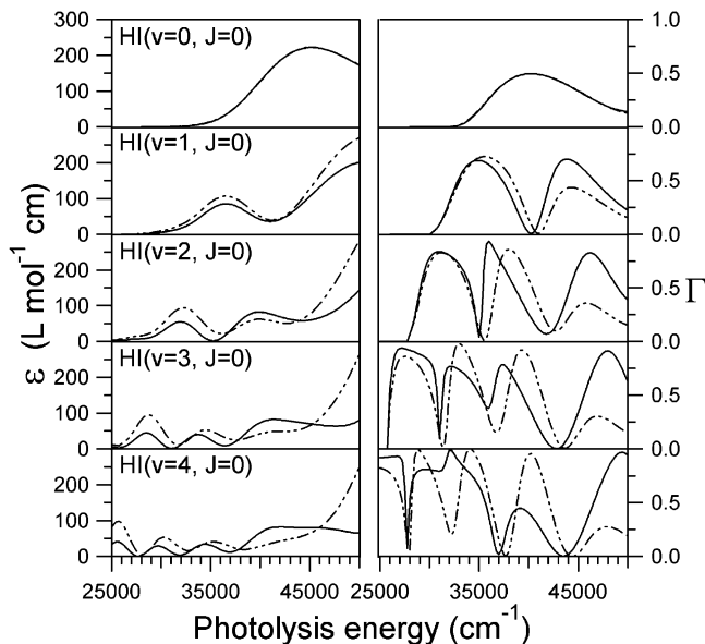
Figure 9. Predicted total absorption cross sections and branching ratios, \Gamma , for HI ( v=0-4, J=0 ) photolysis obtained using model 1 (dash-dot-dot lines) and model 2 (solid lines). The models are indistinguishable in the regions where experimental measurements are available; however, significant differences between the models are observed in the absorption cross sections and branching ratios of higher vibrational states.
