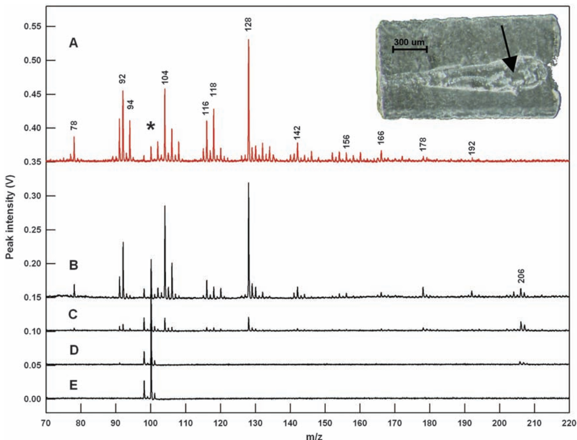
Fig. 1. \mu\text{L}^2\text{MS} mass spectra comparing PAHs detected during laser pulse heating of Stardust witness coupon aerogel to those detected on a cometary impact track. (A) Mass spectrum taken at the entry portion of Wild2 cometary particle impact track (C2115,26,22 track 6); scaled down by a factor of 4. Main m/z peaks are indicated. This distribution consists of aromatic compounds with masses between 78 (benzene) and 178 (phenanthrene) atomic mass units (amu). A series of alkylated components was found for masses 78 amu (benzene), 128 amu (naphthalene), and 178 amu (phenanthrene), as evidenced by mass peaks separated by 14 amu ( \text{CH}_2 ) corresponding to the loss of H and the addition of \text{CH}_3 (Fig. 2A). No PAHs in the area of interest were detected on
