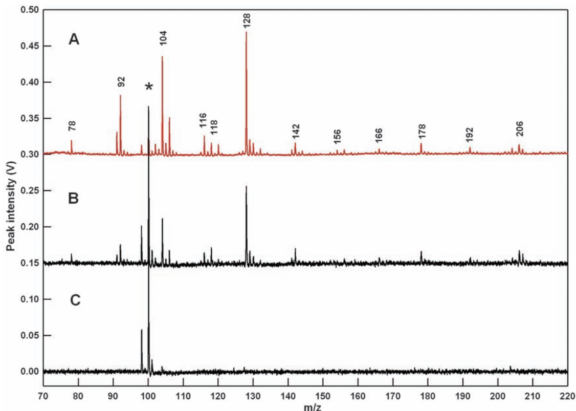
Fig. 2. \mu\text{L}^2\text{MS} mass spectra comparing PAHs detected during laser pulse heating of Stardust witness coupon aerogel to those detected at the same position 14 days later using normal operating parameters, both on and off of the original high-power laser shot position. Main m/z peaks are indicated. The asterisk indicates mass calibration peaks for \text{D}_8 -toluene. (A) Mass spectrum composed of 50 averaged mass spectra taken over the surface of a witness coupon sample (WCARMI1CPN,0,6) at high laser desorption power (two attenuation grids). Prominent peaks include 78 amu (benzene), 92 amu (toluene), and 104 amu (styrene). Masses at 104 amu (styrene) and 128 amu
