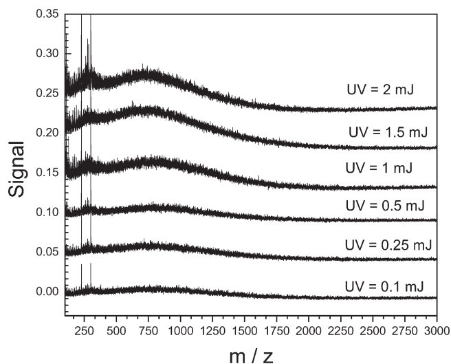
Figure 5. L 2 MS spectra of BG5 asphaltenes recorded at different ionization laser pulse energies using single-photon ionization at 157 nm. Note that the asphaltene average molecular weight is near 600, with an upper limit near 1500.
