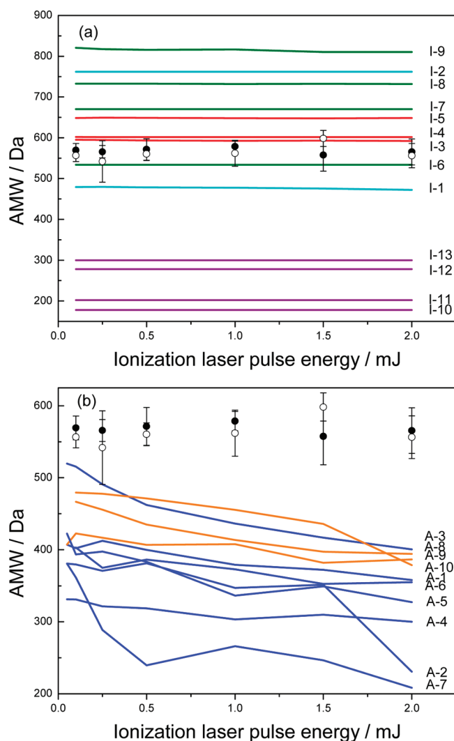
Figure 6. Fragmentation behavior of different compounds as a function of ionization laser pulse energy: (a) island compounds and (b) archipelago compounds. Black dots, BGS asphaltenes; open dots, UG8 asphaltenes; blue lines, linked-pyrene model compounds; orange lines, linked-phenanthrene model compounds; red lines, cholestanones; cyan lines, single-pyrene model compounds; green lines, porphyrins; and purple lines, PAHs.
