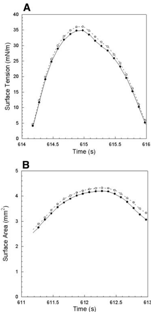
Fig. 7. Comparison of spherical vs. ellipsoidal shape assumption for DPPC at 1.0 mg/ml, 37°C, and 20 cycles/min. A : steady-state surface tension as a function of time. B : surface area (capillary tube area not corrected for) as a function of time. ●, Data assuming an ellipsoid; ○, data assuming a sphere. Loop directions are clockwise.
