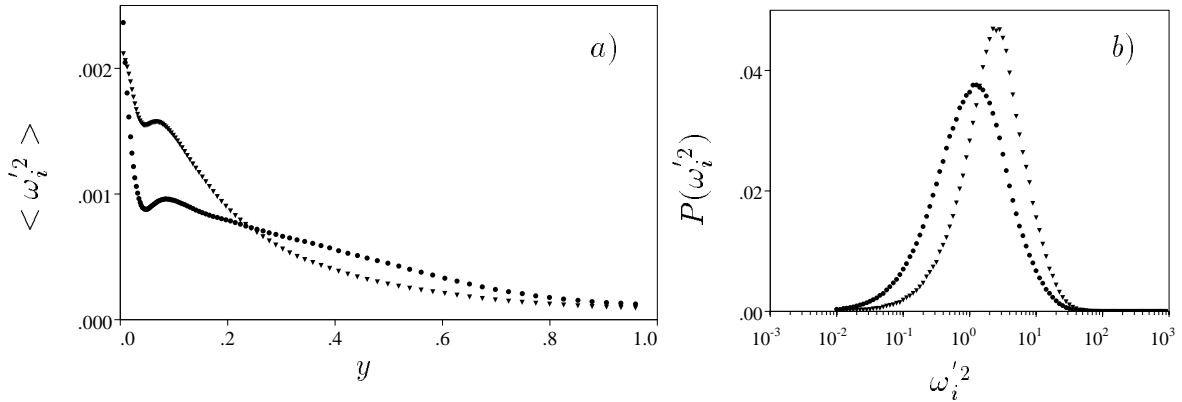
FIGURE 6. a) Dissipation radial profile, b) Probability density function of the local dissipation at y^+ = 10 ; \blacktriangle N = 0 , \bullet N = 2 .
