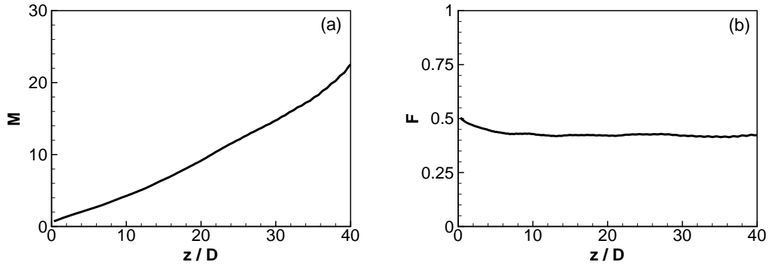
FIGURE 2. Streamwise variation of radially and azimuthally integrated (a) momentum and (b) buoyancy fluxes.
