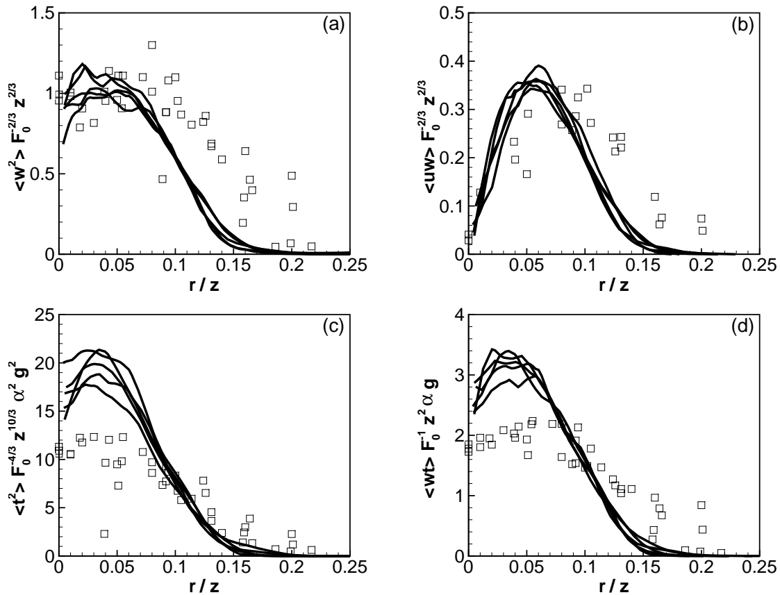
FIGURE 5. Second order moments plotted in terms of similarity variables. (a) the vertical velocity fluctuations, (b) the turbulent shear stress, (c) temperature fluctuations, (d) the vertical turbulent heat flux. The lines represent the computed results at z/D = 20, 25, 30, 35 and 40 ; the experimental data from Shabbir & George (1994) are shown superposed using \square symbols.
