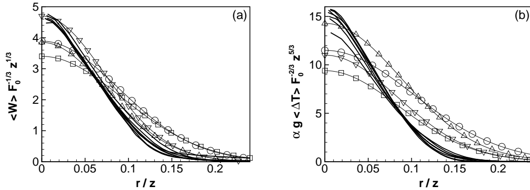
FIGURE 4. Radial profiles of (a) mean streamwise velocity and (b) mean temperature difference plotted in similarity form. The computed results at z/D = 15 to 40 at interval of 5 are shown using bold lines. The lines with symbols represent the experimental data as described in Fig. 3.
