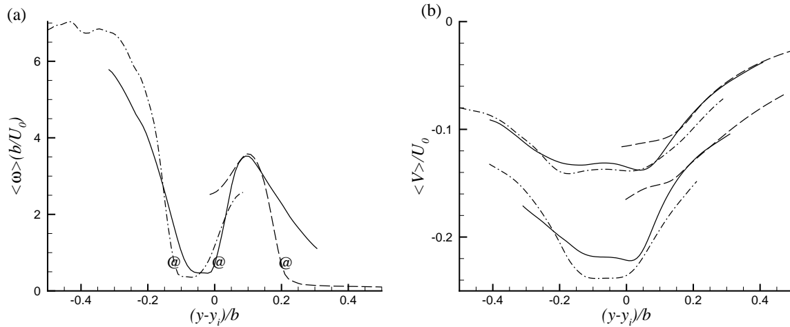
FIGURE 5. Conditional results for re-entrant zones. Surfaces: ----, outermost; —, downwards-facing; - · - ·, innermost. (a) \langle \omega \rangle , unforced wake. (b) Corresponding distributions of \langle V \rangle , unforced (upper curves) and forced (lower curves).
