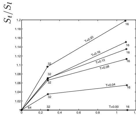
FIGURE 8. Ratio of the resolved DNS flame area to the filtered flame area as a function of the subgrid kinetic energy u' at various filter levels. Results for passive G -field with higher order upwind method.
