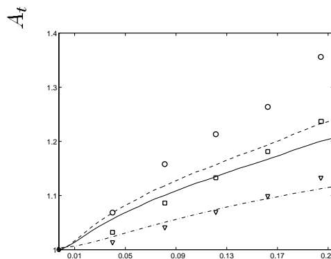
FIGURE 7. Turbulent flame speed as a function of time from various DNS/LES calculations obtained with higher order upwind scheme. DNS results: 64^3 , \circ ; 32^3 , \square ; 16^3 , \nabla . LES results: 64^3 , ----; 32^3 , —; 16^3 , -.-.
