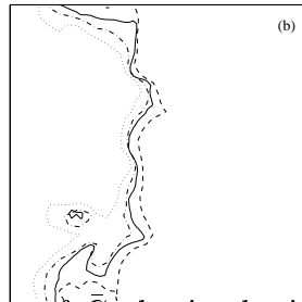
FIGURE 3. The contours of \bar{G} obtained with various LES models after one eddy-turnover time; (a) \bar{G} = 1.45 which is the average value and (b) \bar{G} = 1.95 . A single slice in 3-D is shown. In each figure, DNS result: ——— ; model A: - - - - ; model B: ······ ; model D: — · — · . Flame propagates from right to left.
