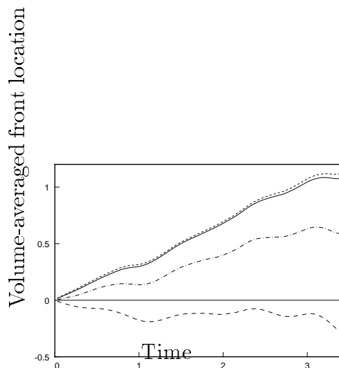
FIGURE 4. The volume-averaged front location according to DNS and various LES models; model A: ---- ; model B: — ; model C: ..... ; model D: —·— .
