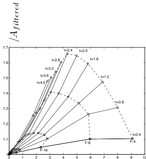
FIGURE 1. Ratio of the resolved DNS flame area to the filtered flame area as a function of the subgrid kinetic energy u' . DNS data by Trouvé & Poinot (1994).
