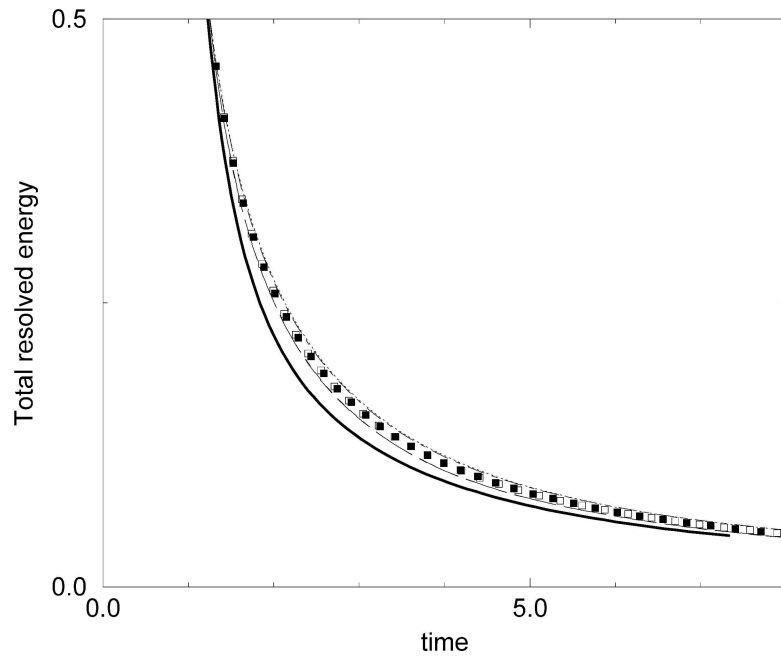
FIGURE 3. Energy decay: comparison with DNS and volume average. DNS:— ; ensemble-averaged (mean): \square ; ensemble-averaged (mean+sigma):- - - ; ensemble-averaged (mean-sigma):- - - ; volume-averaged (mean): \blacksquare ; volume-averaged (mean+sigma): \cdots ; volume-averaged (mean-sigma):- . - .
