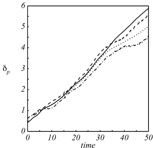
FIGURE 3. Product thickness for S = 1 (—; not affected by the asymmetry) and for S = 8 (— —) and 1/8 (---), corresponding to a flip experiment, for \epsilon = 0.45 , Re = 500 and Pr = 1 . ..... : common value for S = 8 and 1/8 when \epsilon = 0 .
