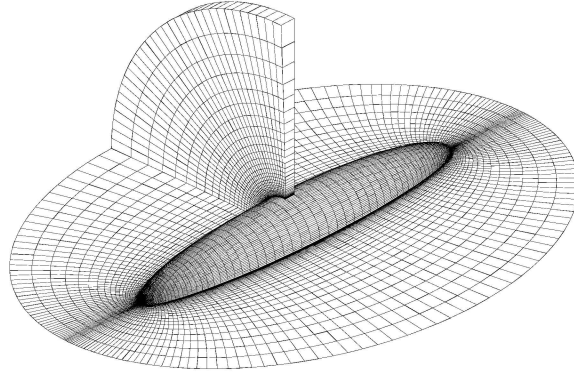
FIGURE 11. Prolate spheroid: geometry and partial grid
